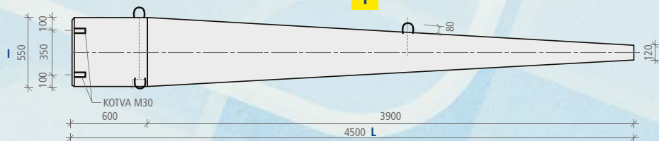
POHLAD ZHORA
